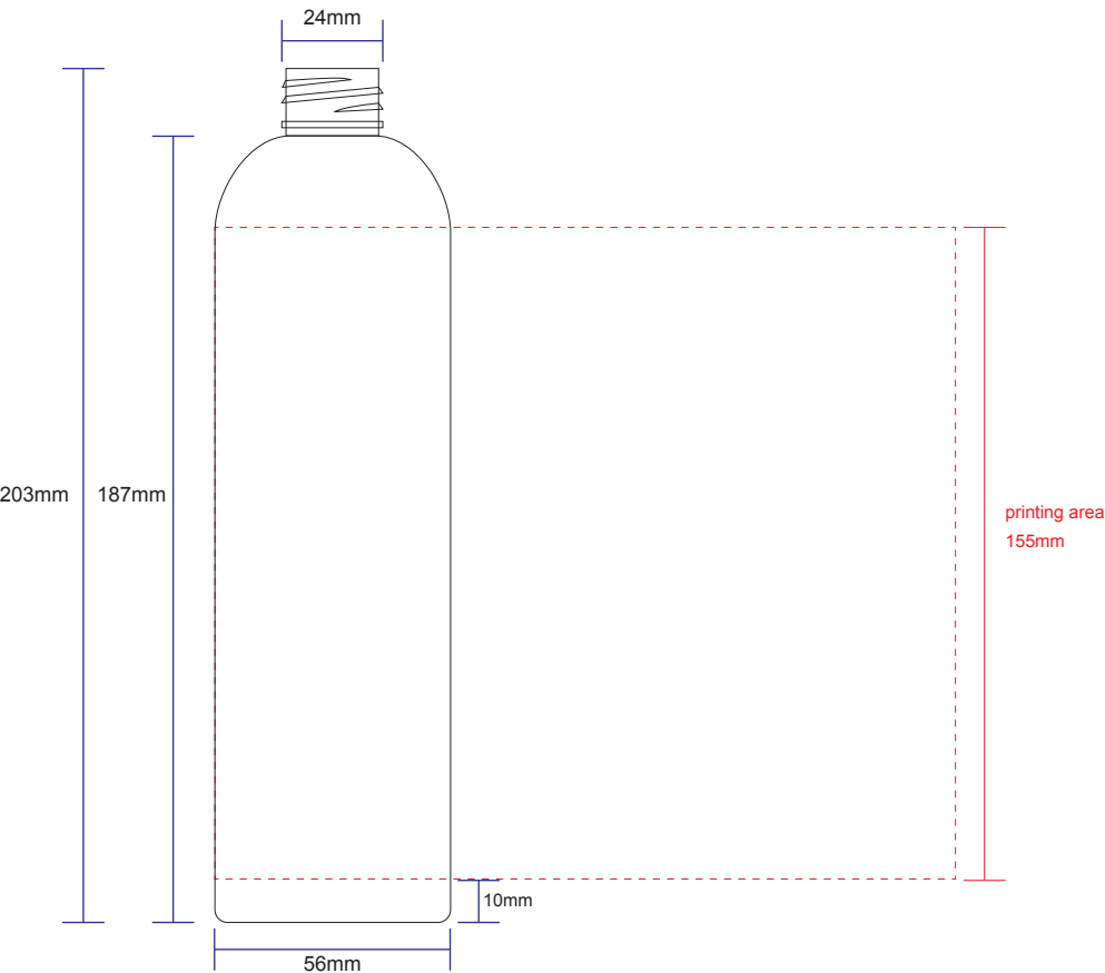
FRONT VIEW
