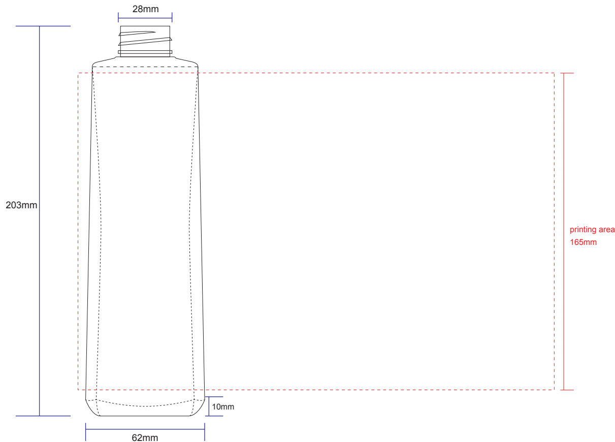
FRONT VIEW
